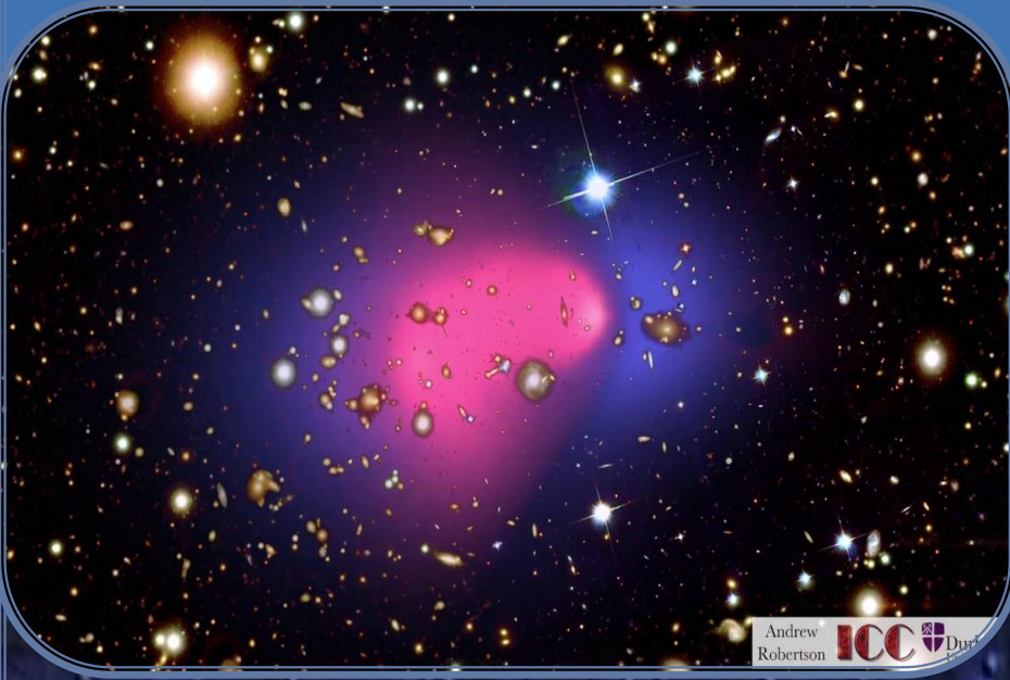
Bullet Cluster
