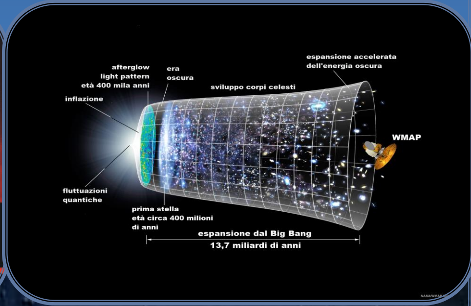
Evolution history of the Universe
